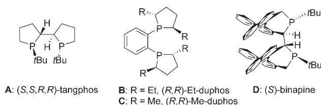
Scheme 1. Chiral ligands for asymmetric hydrogenation.
